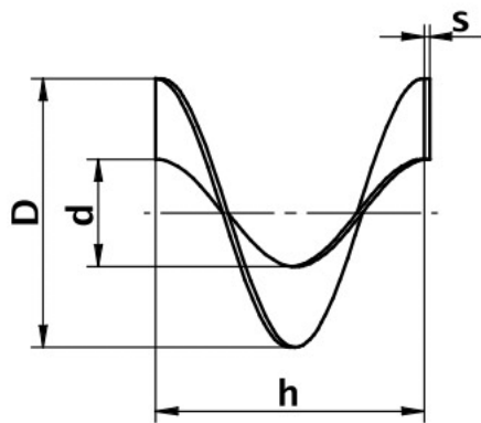
right-hand thread
